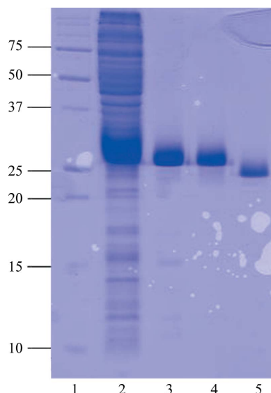
Figure 1 SDS-PAGE analysis of the purification steps of the spinach recombinant PsbP protein. Lane 1, molecular-weight markers (kDa); lane 2, supernatant after IPTG induction of B152 cells; lane 3, the His-tagged PsbP protein purified by metal-affinity chromatography; lane 4, His-tagged PsbP protein purified by ion-exchange chromatography; lane 5, recombinant PsbP protein after Superdex 75 column chromatography.
