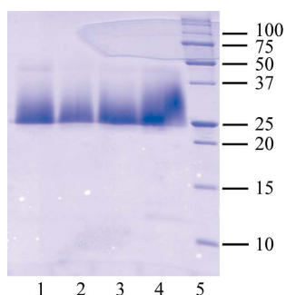
Figure 4 SDS-PAGE analysis of dissolved PsbP crystals obtained from four different conditions: lane 1, 20% PEG 550 MME, 0.1 M Tris-HCl pH 7.0, 20 mM ZnCl 2 ; lane 2, 15% PEG 550 MME, 0.1 M Tris-HCl pH 7.0, 20 mM ZnSO 4 ; lane 3, 15% PEG 550 MME, 0.1 M Tris-HCl pH 7.5, 20 mM ZnSO 4 ; lane 4, 15% PEG 8000, 0.1 M Tris-HCl pH 7.5, 20 mM ZnCl 2 ; lane 5, molecular-weight markers (kDa).
